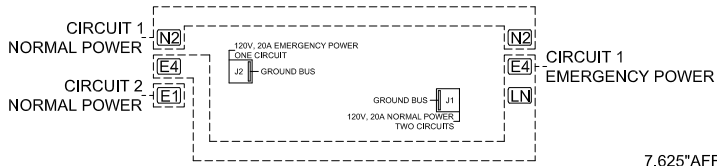
WIRING DIAGRAM
