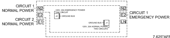
WIRING DIAGRAM
